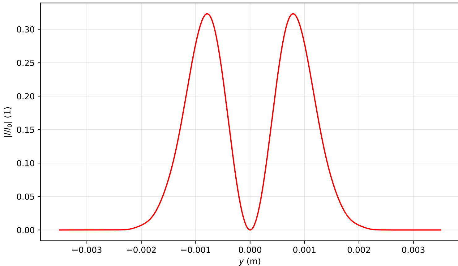
Intensity profile I(x=0, y, z=2.627)/I_0 , P_{in}=1.0P_{cr} , artificial time
